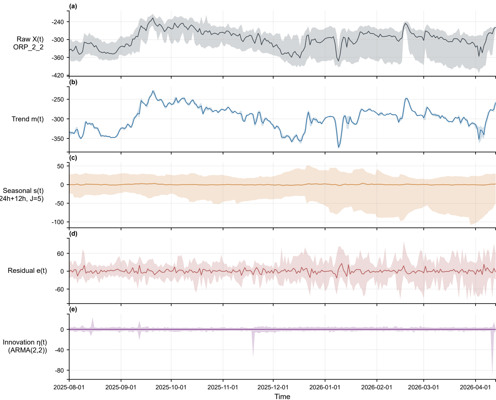
Full-span daily overview — ORP_2_2 (pre_anoxic_front, min) [2025-08-01~2026-04-13]
